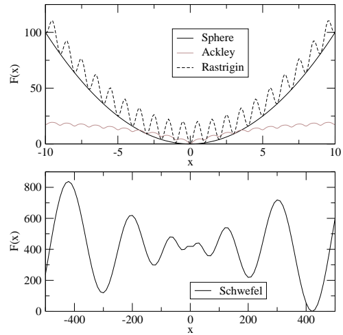
Figure 2: Sphere, Ackley and Rastrigin (top) and Schwefel (down) functions in one-dimensional problem N = 1 .
