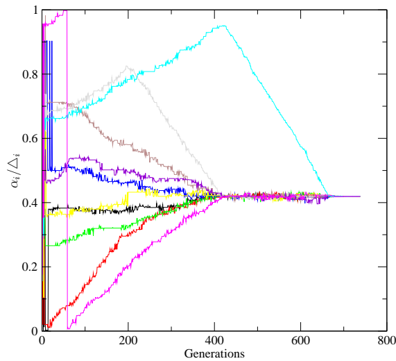
Figure 5: Convergence history of a typical run of Schwefel function: \alpha_i/\Delta_i ratios of the best individual.
