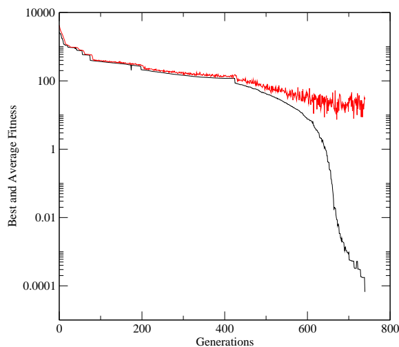
Figure 3: Convergence history of a typical run of Schwefel function: fitness of the best individual and population average fitness.
