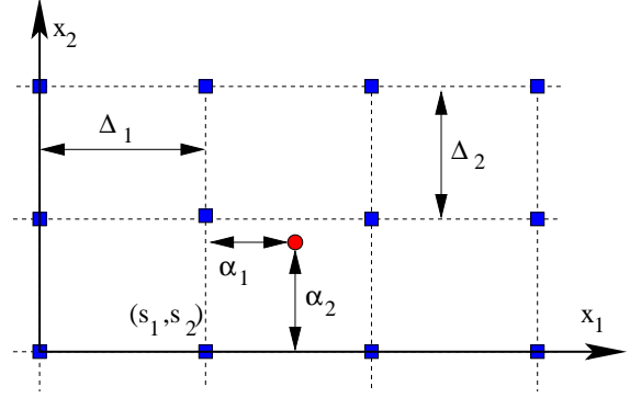
Figure 1: Graphical example of encoding in a two-dimensional problem. The point represents an individual, being its relative coordinates (\alpha_1, \alpha_2) respect to the grid node (\Delta_1 s_1, \Delta_2 s_2) . The absolute coordinates are (s_1 \Delta_1 + \alpha_1, s_2 \Delta_2 + \alpha_2) where \Delta_1 and \Delta_2 are the grid step sizes in each dimension.
