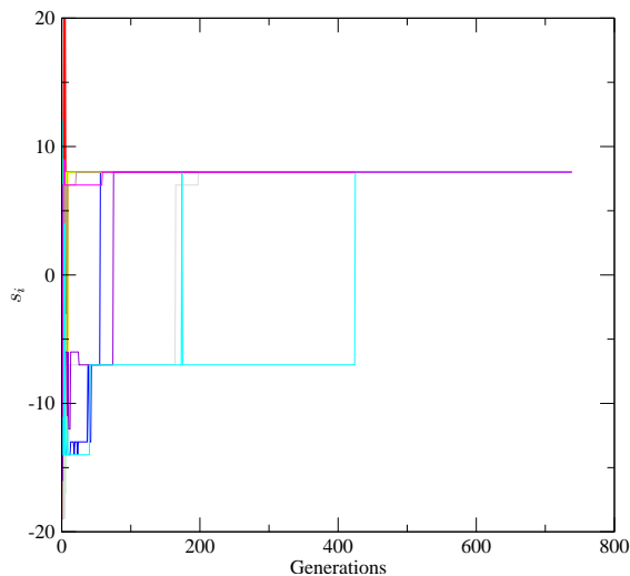
Figure 4: Convergence history of a typical run of Schwefel function: steps s_i of the best individual.
